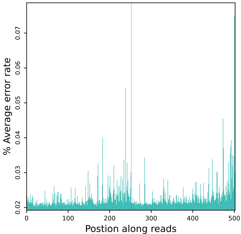
Error rate distribution along reads (R10516)
